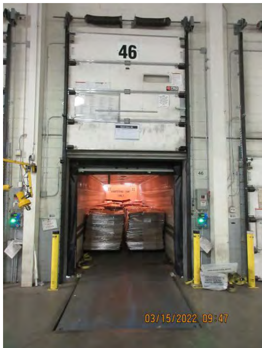
DOOR 46 Remove Existing Red/Green Light System
