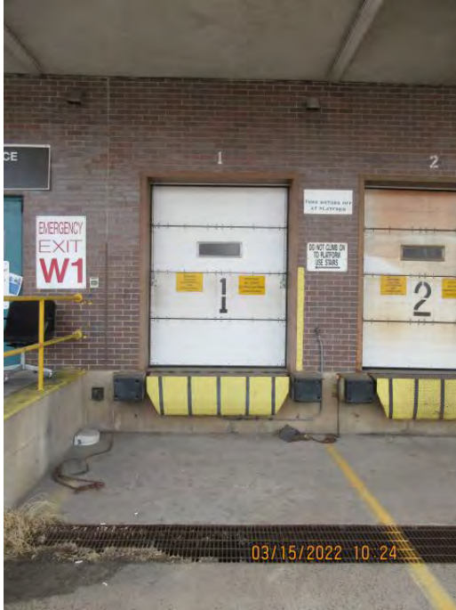
DOOR 1 Install Kelley Dock Communication System
