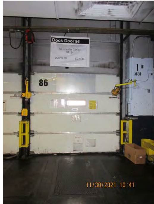
DOOR 86 Remove Existing Red/Green Light System
